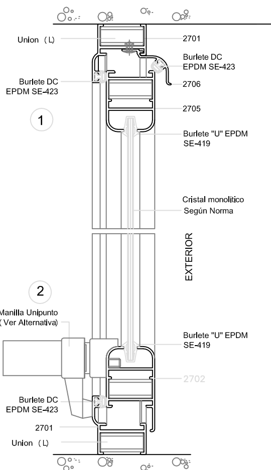
CORTE VERTICAL
